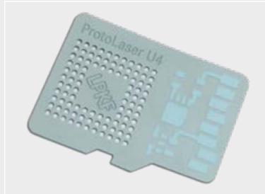
Structuring, engraving, drilling, and depaneling: the ProtoLaser U4 can also be used to process LTCC ceramics
