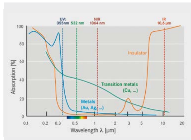
The absorption values vary according to laser wavelength and material
