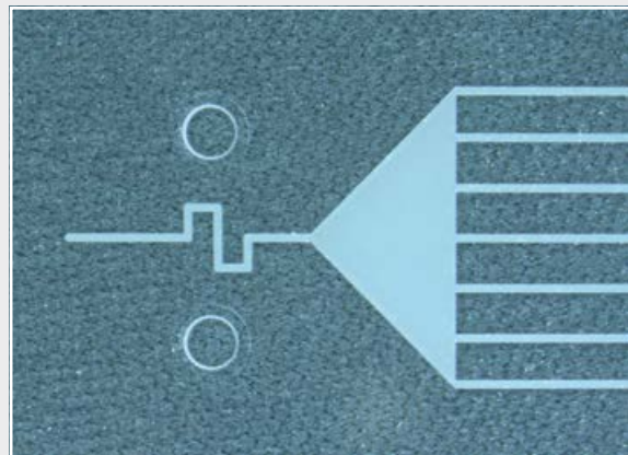
Processing stretchable flex PCB for wearables, deep engraving of PI for microfluidics
